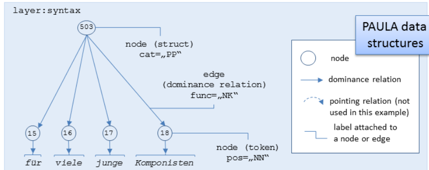
Fig. 2 Constituent syntax: Fragment from Fig. 1 with PAULA data structures.
